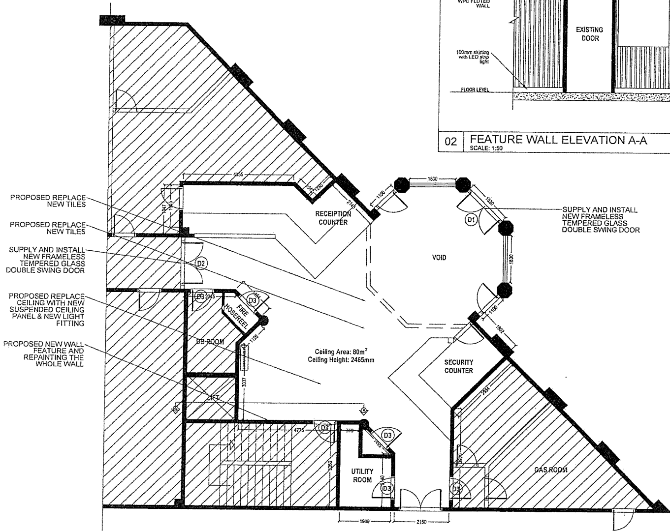
01 GROUND FLOOR LOBBY SCALE: 1:100
